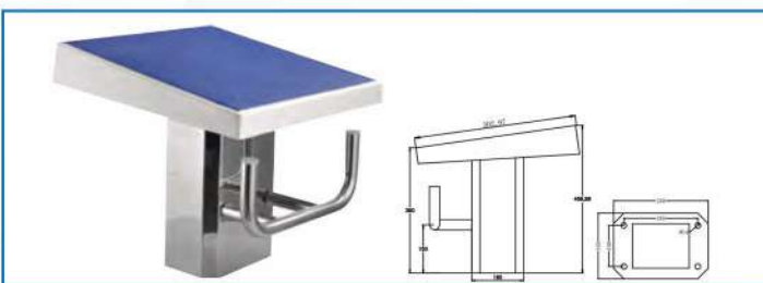
HVTP-301 STANDARD ONE-STEP STARTING BLOCK
