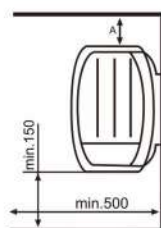
Installation dimension
