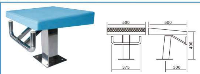
HVTP-303 STANDARD ONE-STEP STARTING BLOCK
