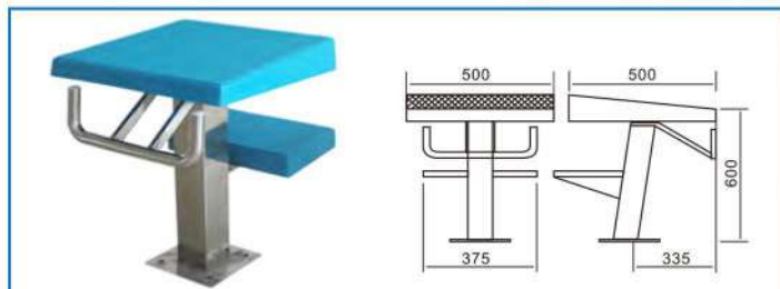
HVTP-305 STANDARD TWO-STEP STARTING BLOCK
