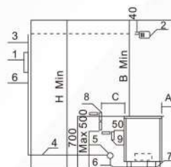
Installation dimension
