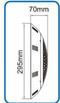
HPK6004 Wall Mounted Type Pool Light
